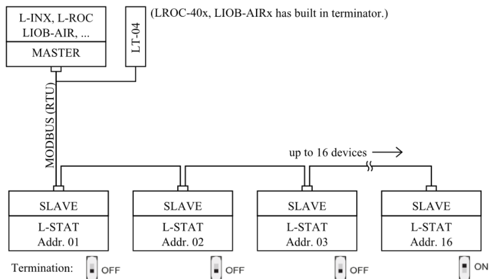
Figure 7: Modbus Network
