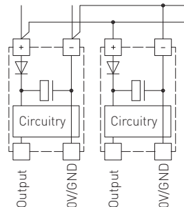
Parallel operation
