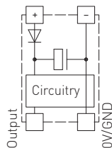
Individual operation
