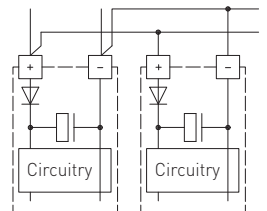
Parallel operation
